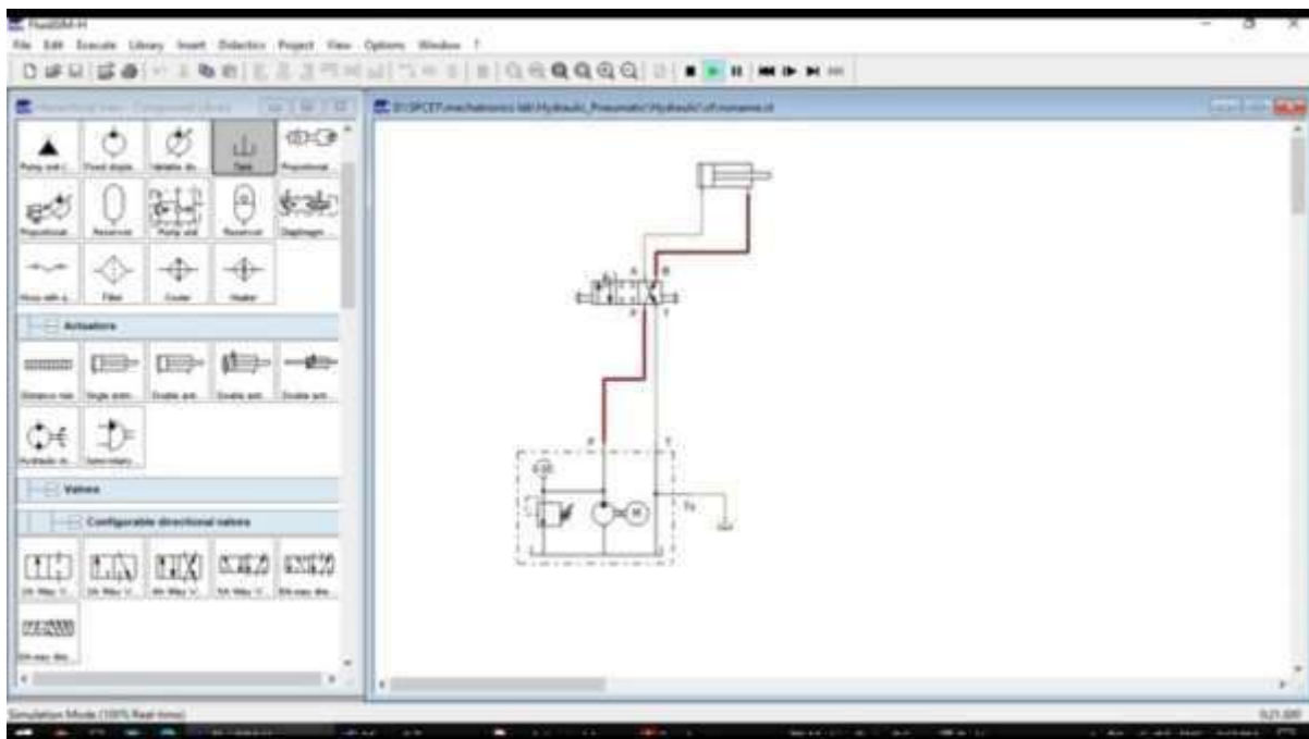
simulation of working of double acting cylinder using FluidSIM
