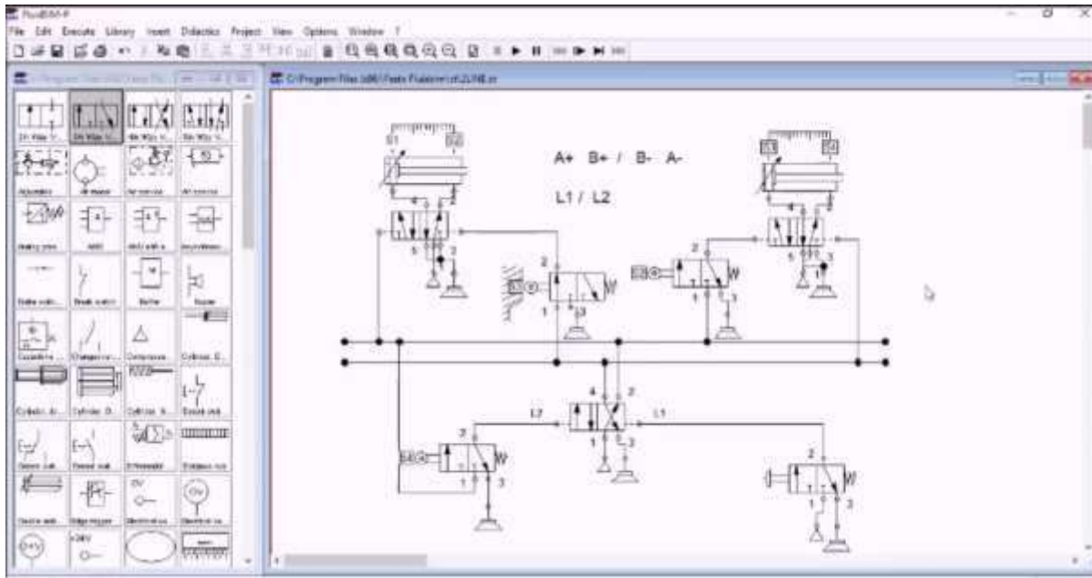
simulation of working of Cascade Circuit using FluidSIM
